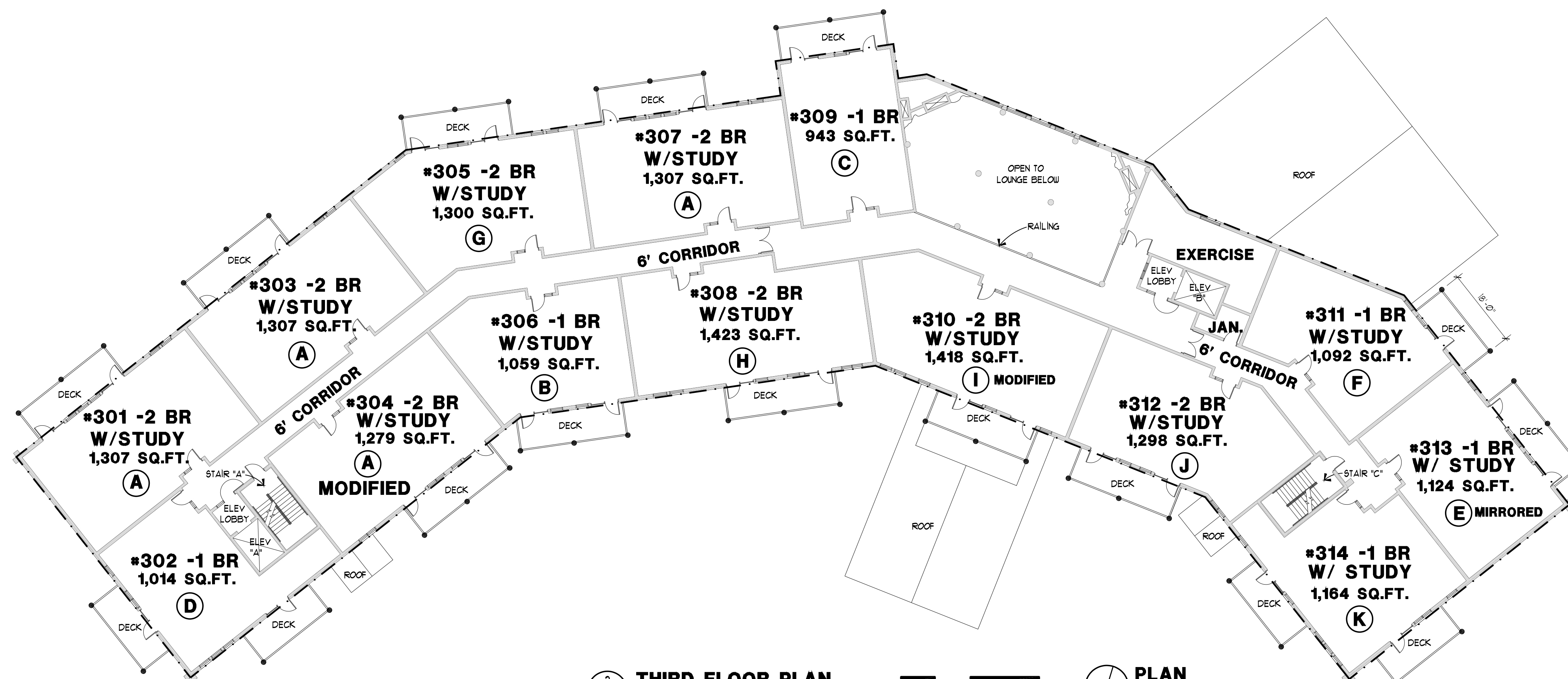
2 THIRD FLOOR PLAN PLAN NORTH
